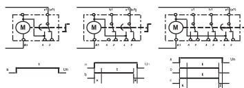
Switching program
