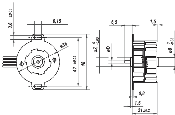
Dimensions Mounting with screw plate
